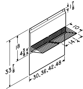
Restaurant-quality stainless steel backsplash with fold-down shelves completes the commercial look and is easy to clean.
