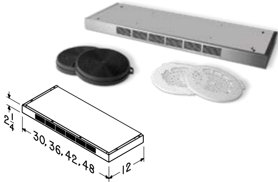
A non-duct kit may be used to recirculate filtered air back into the kitchen if ducting is not practical.
